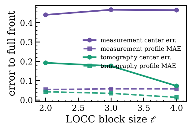
(f) LOCC improves with \ell
