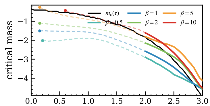
(b) DPT mass vs time
