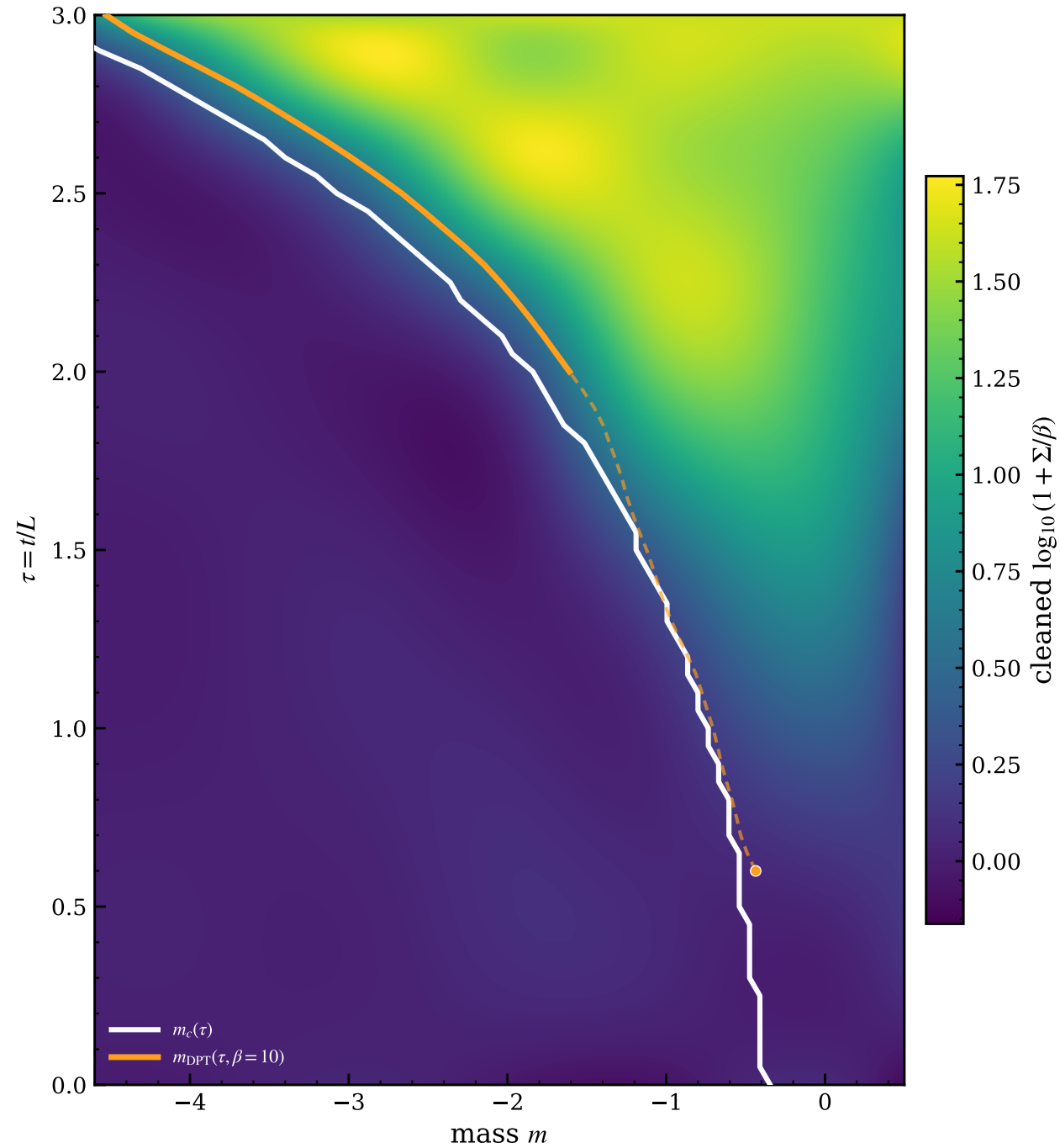
(a) Front at \beta=10
